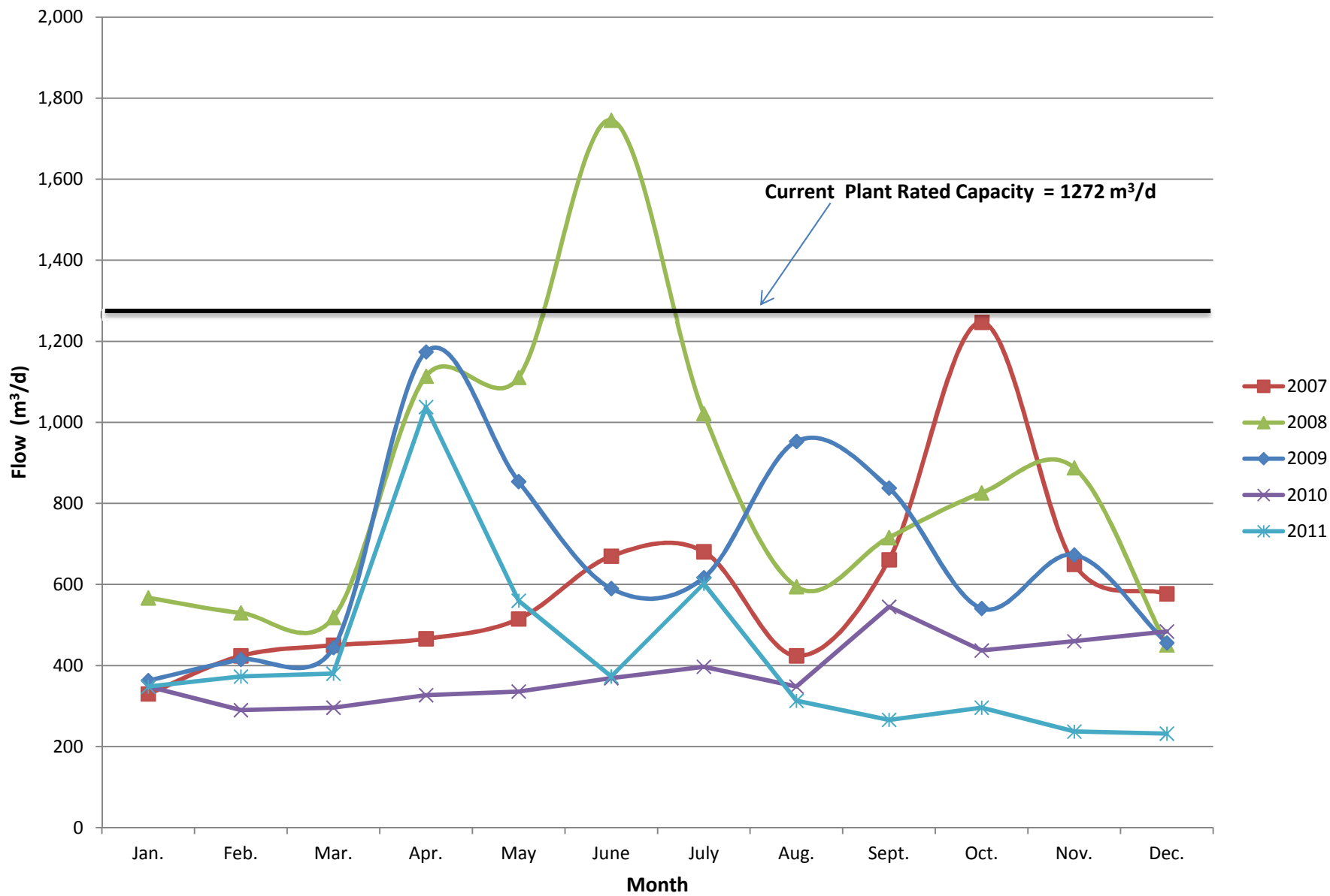
Figure 2.2: Red Rock WWTP Historical Average Daily Flows
